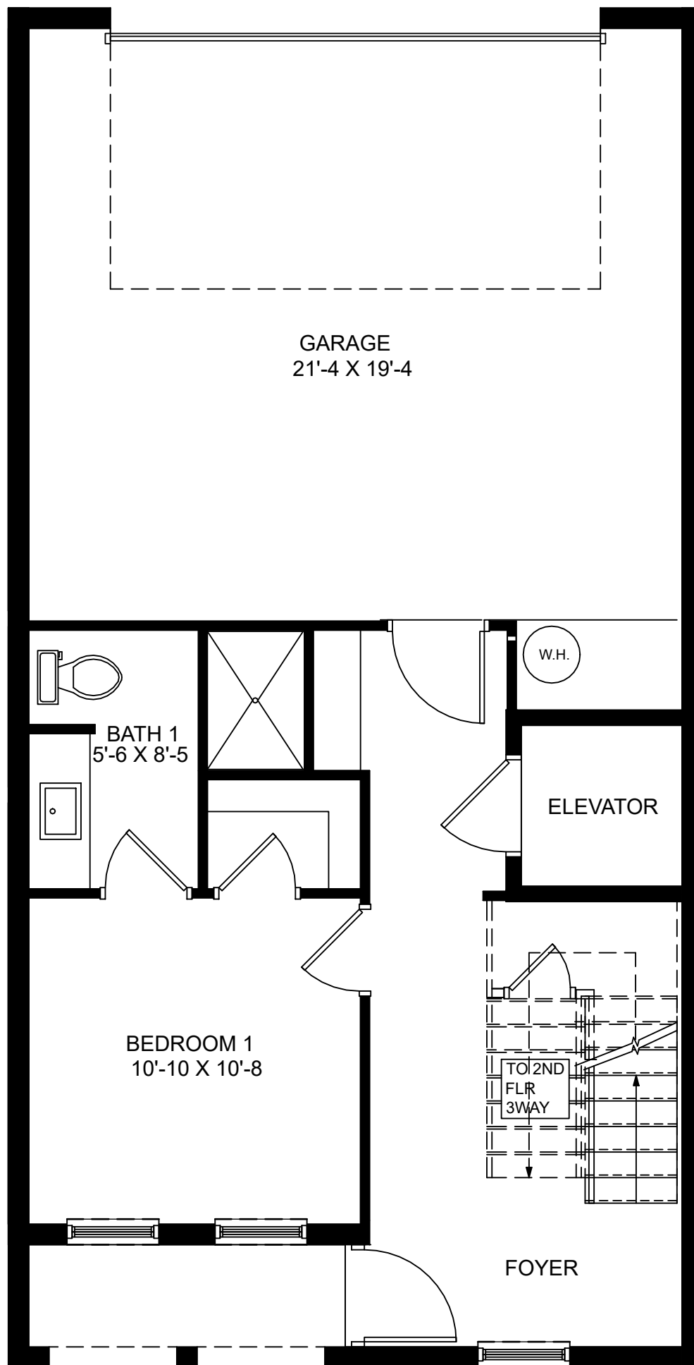
FIRST FLOOR PLAN UNIT 17
