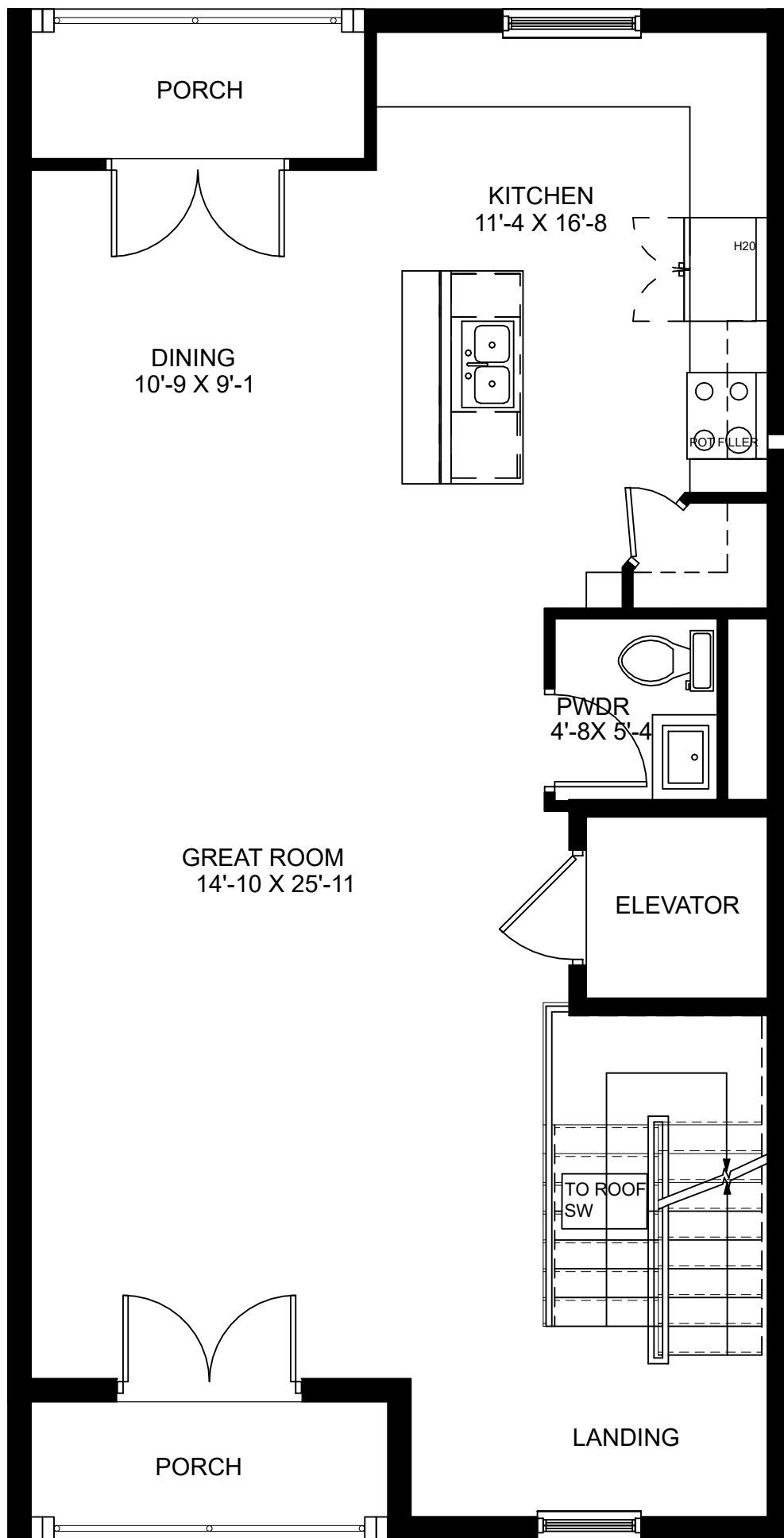
THIRD FLOOR PLAN UNIT 17
