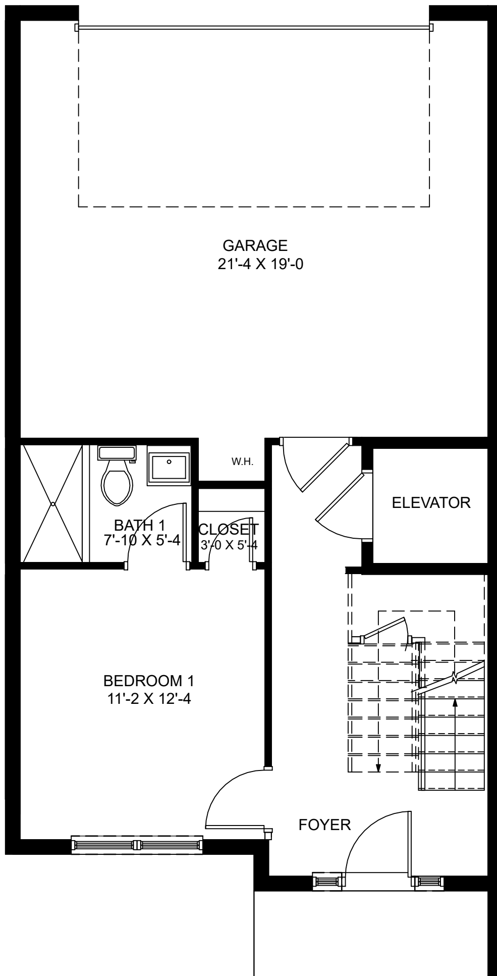
FIRST FLOOR PLAN UNIT 16
